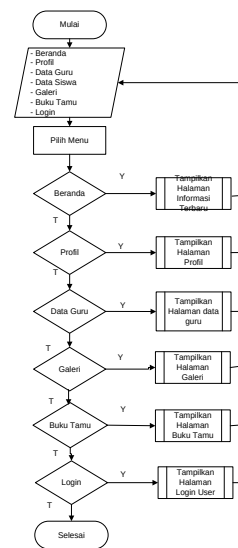
Gambar 3.6 Flowchart Login
