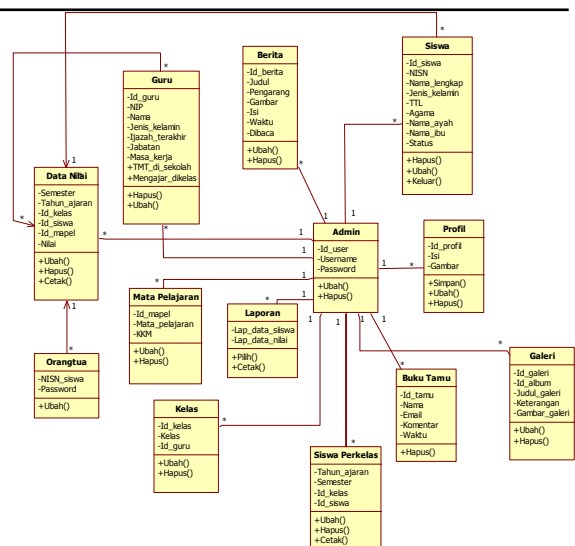
Gambar 3.2 Class Diagram
