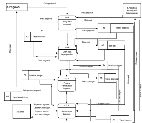
Gambar 4.2 Overview Diagram (Level 0)
