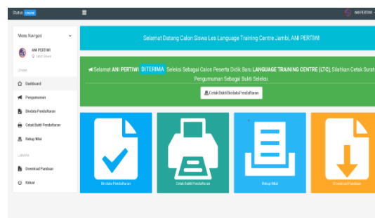
Gambar 6. Tampilan Dashboard
