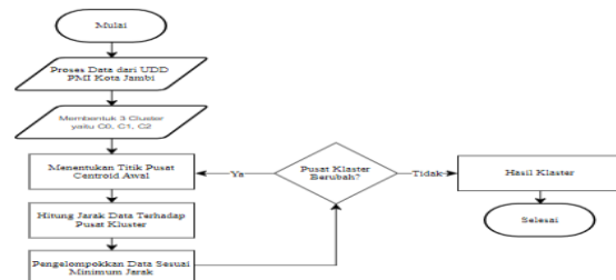
Gambar 1. Proses perhitungan K-Means
