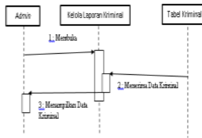
Gambar 9. Sequence Diagram Admin Kelola Laporan
